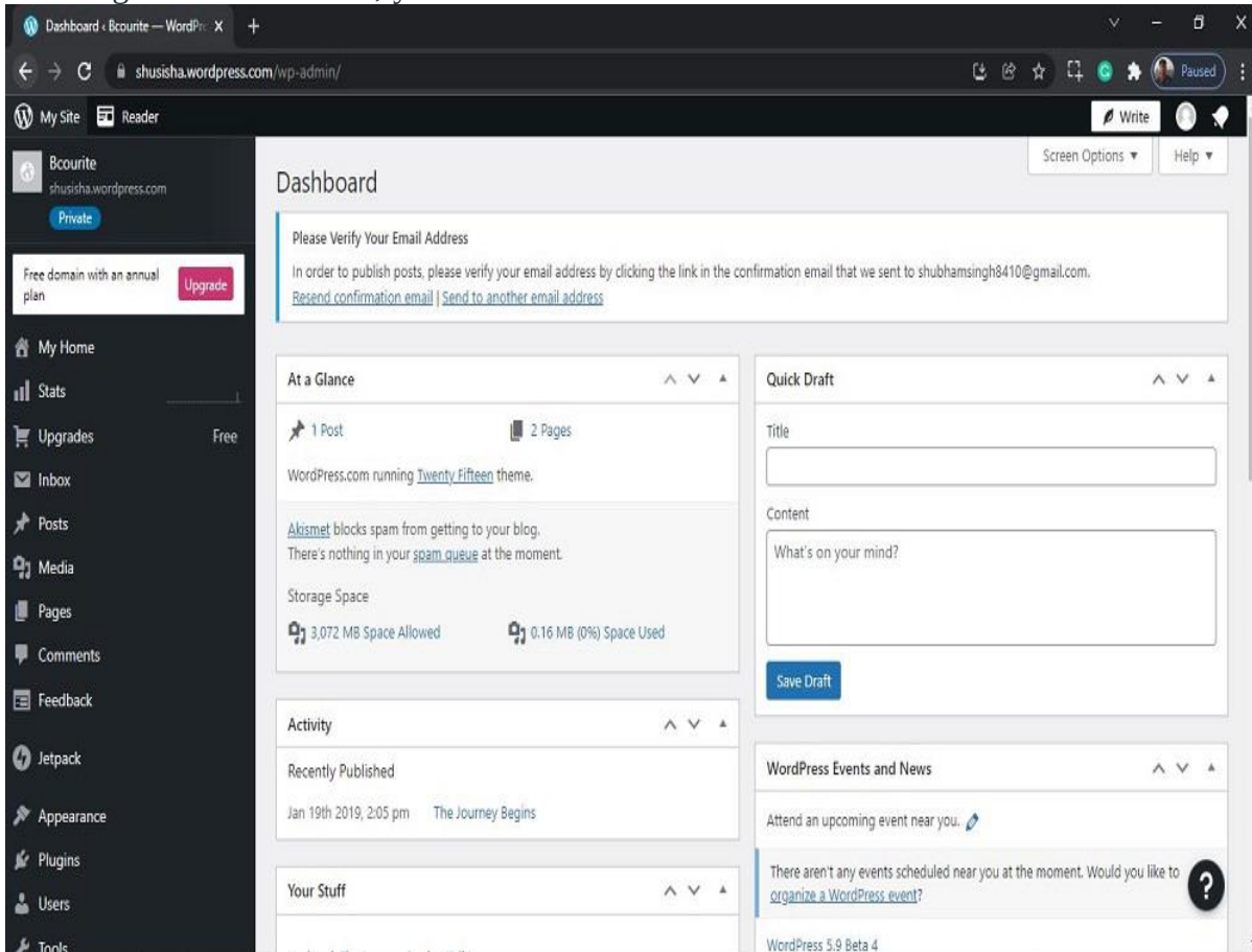
WordPress Dashboard
