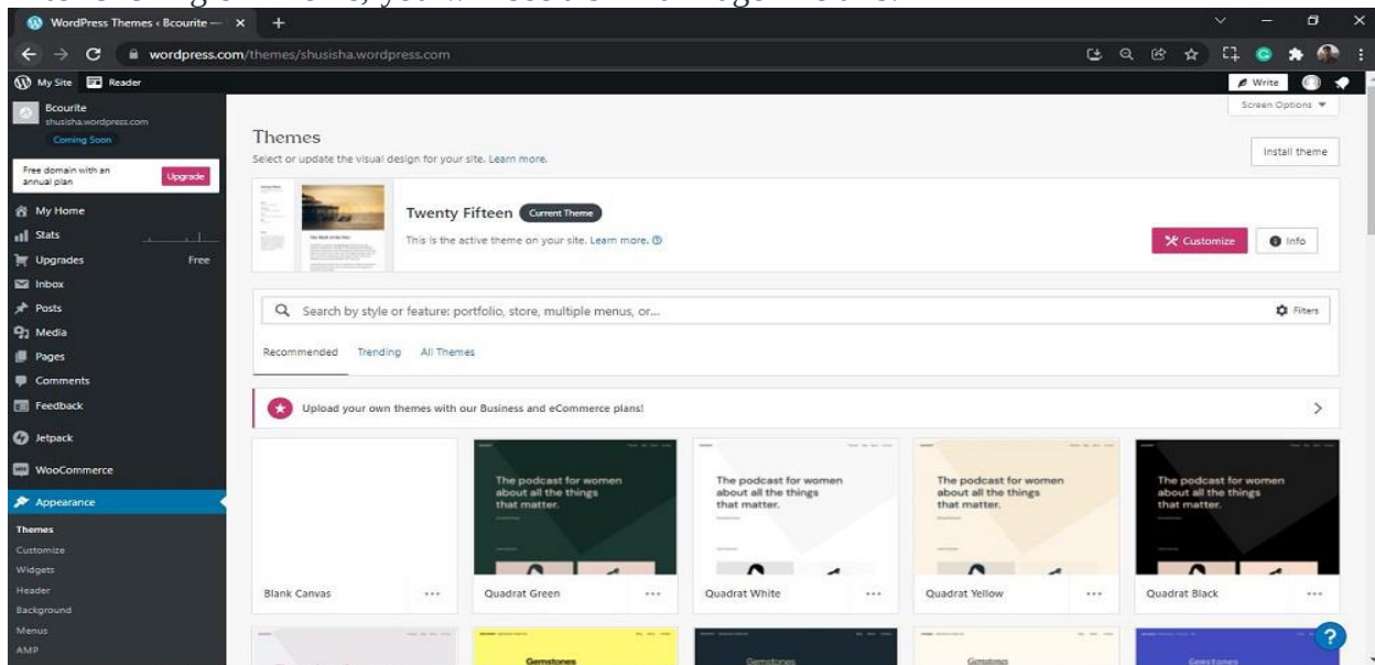
Theme Section
